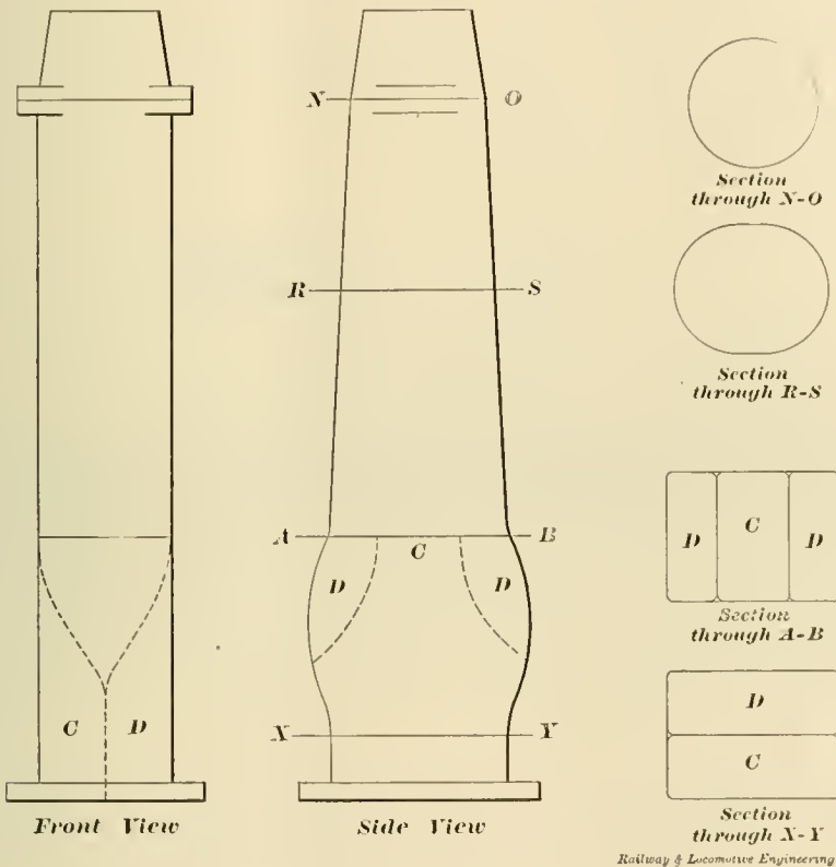
AN EXHAUST NOZZLE THAT WILL NOT CROSS-FIRE.
